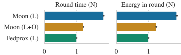
Fig. 9: Normalized (N) round level metrics for Moon and FedProx using an 11.6M parameter model (L), with the addition of a small optimization (O) to the original Moon baseline code. Results show average round data statistics over 30 rounds, with error bars indicating the 95th percentiles.
