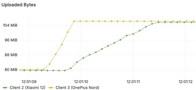
Fig. 11: Uploaded bytes over time after a round of training on FEMNIST dataset [87] using CNN model.
