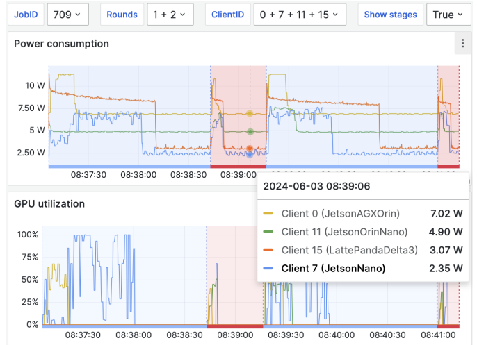
Fig. 3: Example capture of COLEXT Dashboard.
