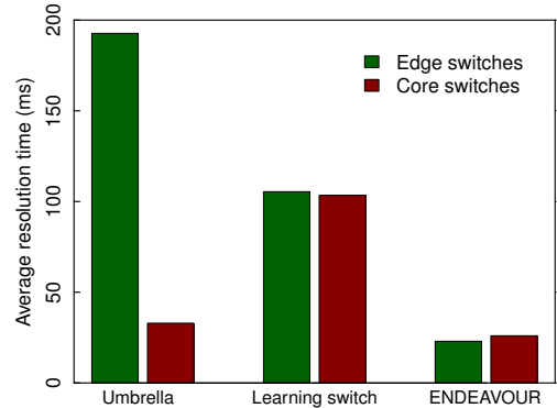
Fig. 7. Average resolve time on switch failure.
